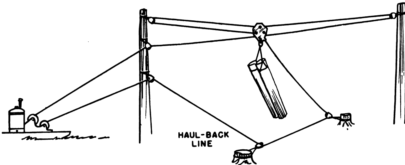
HAULBACK BLOCK
